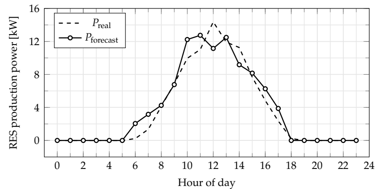
Figure 3. RESPOND production forecasting service output performance for an Aarhus photovoltaic (PV) array.
