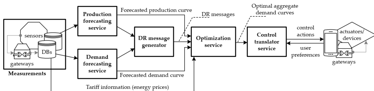
Figure 1 - AI-based control loop
