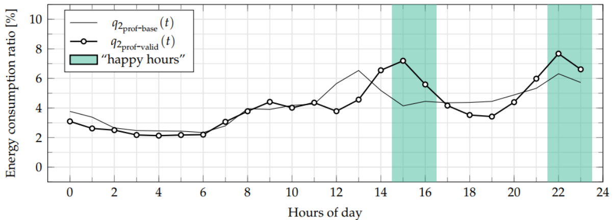
Figure 5 - Visual comparison between hourly demand profiles
