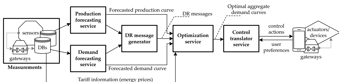
Figure 2. The RESPOND Artificial Intelligence (AI) system loop.
